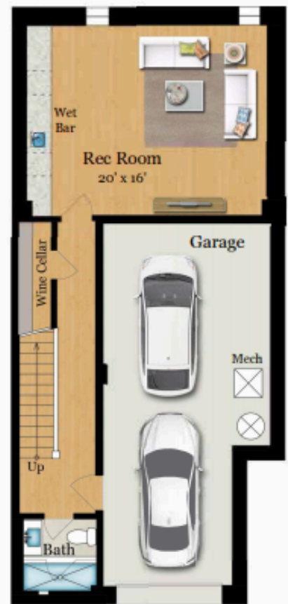
LOWER LEVEL 660 SQ FT
